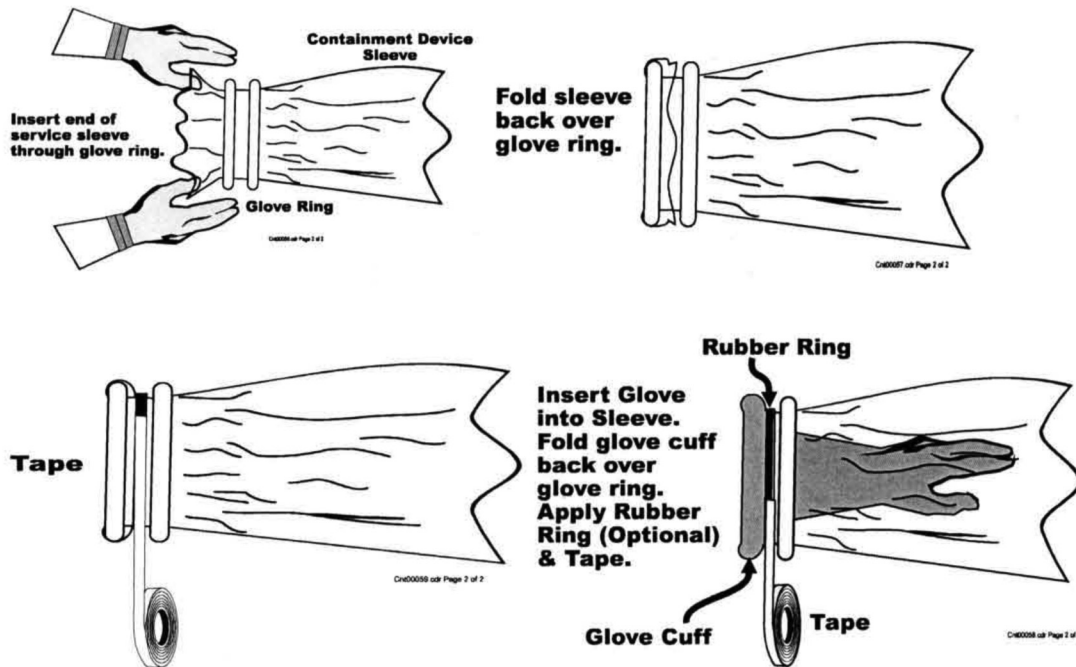
Figure 3. New Glove Installation
